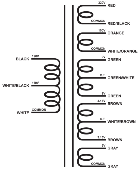
Schematic
